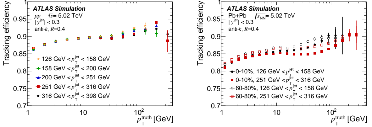
Figure 1: Tracking efficiency, \varepsilon , smoothed using a third-order polynomial in \log(p_T^{\text{truth}}) as a function of p_T^{\text{truth}} in pp collisions in five different jet- p_T intervals (left) and in Pb+Pb collisions (right) in two different jet- p_T intervals and for 0–10% and 60–80% centrality intervals. In both plots the efficiency is evaluated for tracks within jets with |y^{\text{jet}}| < 0.3 .
