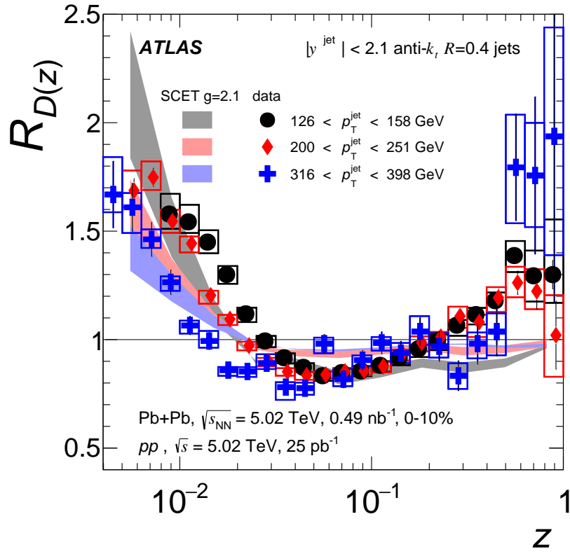
Figure 22: R_{D(z)} for three p_T^{\text{jet}} ranges: 126–158 GeV (circles), 200–251 GeV (diamonds) and 316–398 GeV (crosses) compared with calculations from the SCET model [52, 53].
