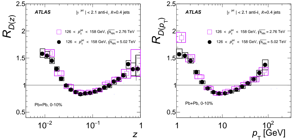
Figure 18: R_{D(z)} (left) and R_{D(p_T)} (right) for 126–158 GeV jets for collision energies of 5.02 TeV (this analysis) and 2.76 TeV [13]. The vertical bars on the data points indicate statistical uncertainties while the boxes indicate systematic uncertainties.
