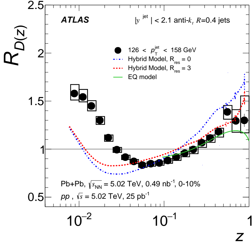
Figure 20: R_{D(z)} for jets with 126 < p_T^{\text{jet}} < 158 GeV compared with calculations from Ref. [48] (Hybrid model) for R_{\text{res}} = 0 (dot-dashed curve), R_{\text{res}} = 3 (dashed curve), and to calculations from Ref. [18] (EQ model).
