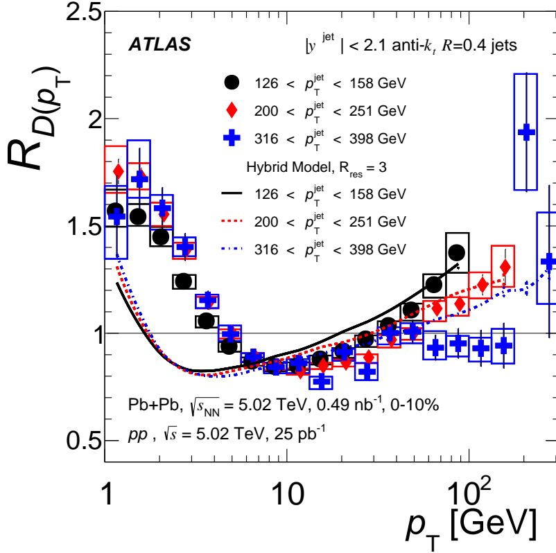
Figure 21: R_{D(p_T)} ratios for three p_T^{\text{jet}} ranges: 126–158 GeV (circles), 200–251 GeV (diamonds) and 316–398 GeV (crosses) compared with calculations from the hybrid model [48] with R_{\text{res}} = 3 .
